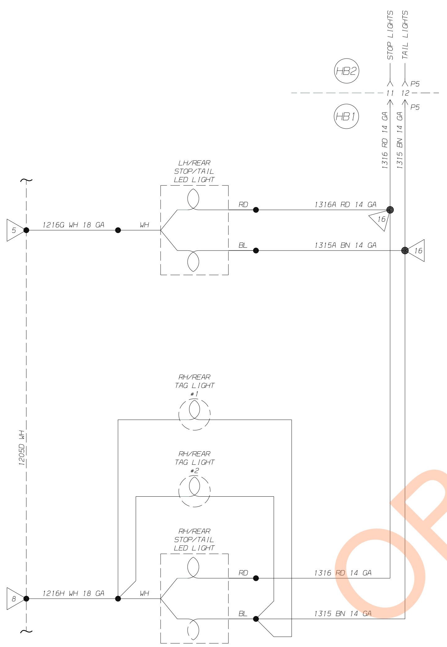
4" LED STOP/TAIL LIGHTS, RH LED TAG LIGHTS FEATURE 30173-07
